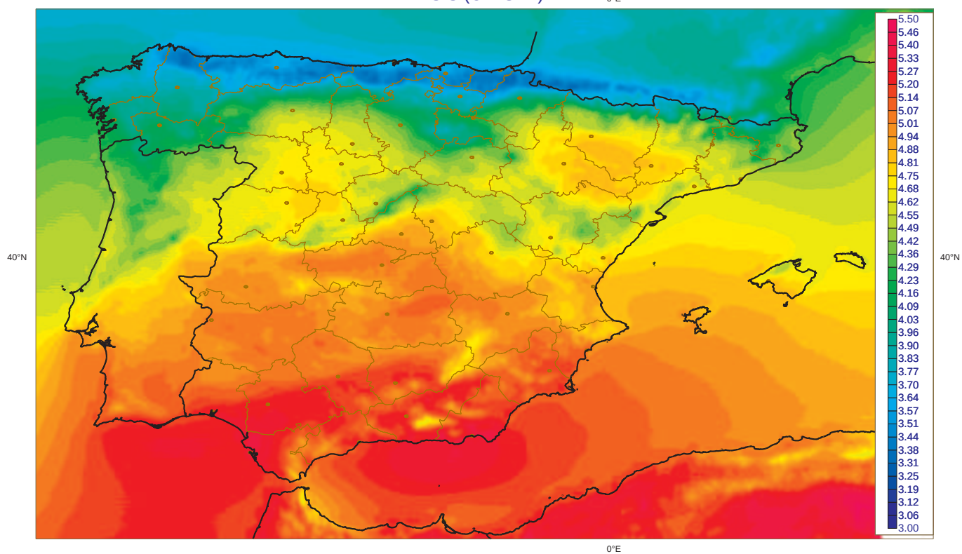
Irradiancia Global media [1983-2005] (Kwh m-2 dia-1) SIS (CM-SAF)
