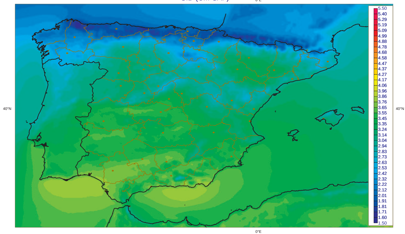
Irradiancia Directa media [1983-2005] (Kwh m-2 dia-1) SID (CM-SAF)
